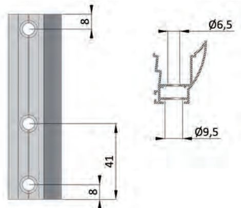
Arrangement of fixing holes
